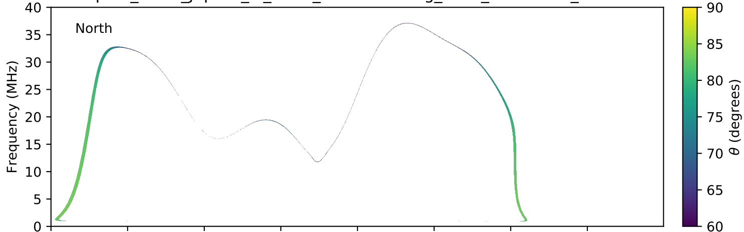
expres_earth_jupiter_io_isaac_lossc-wid1deg_3kev_20170517_v01.cdf
