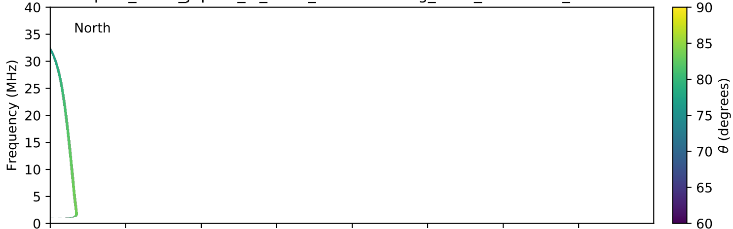
expres_earth_jupiter_io_isaac_lossc-wid1deg_3kev_20170516_v01.cdf
