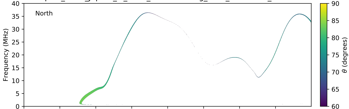
expres_earth_jupiter_io_isaac_lossc-wid1deg_3kev_20170515_v01.cdf
