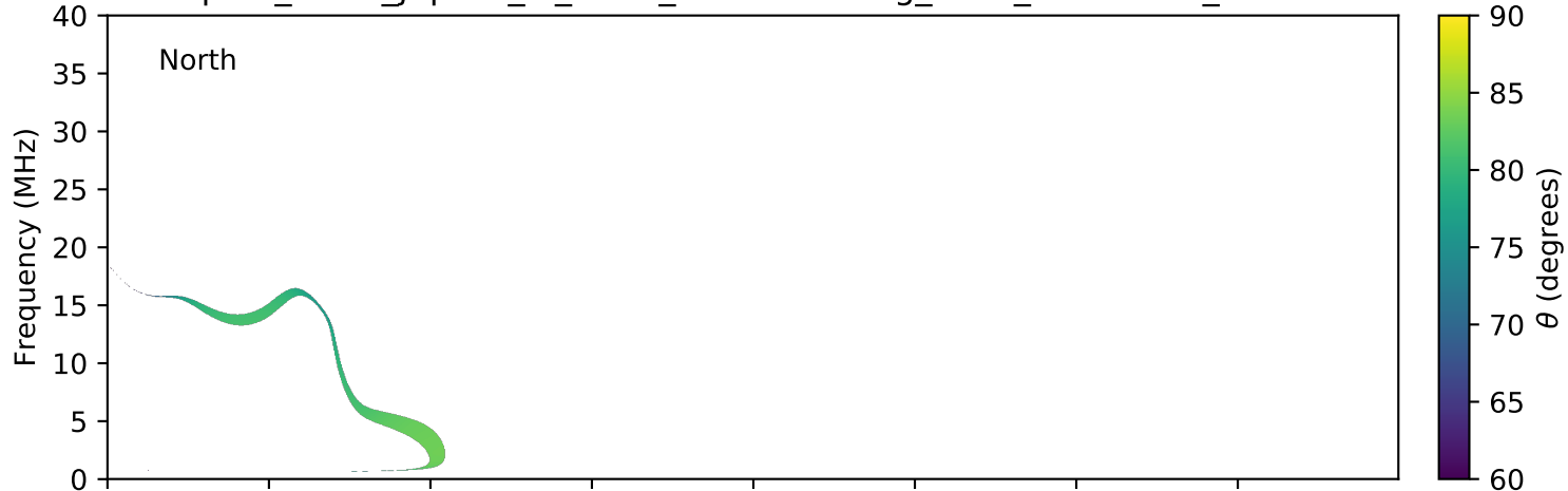
expres_earth_jupiter_io_isaac_lossc-wid1deg_3kev_20170514_v01.cdf
