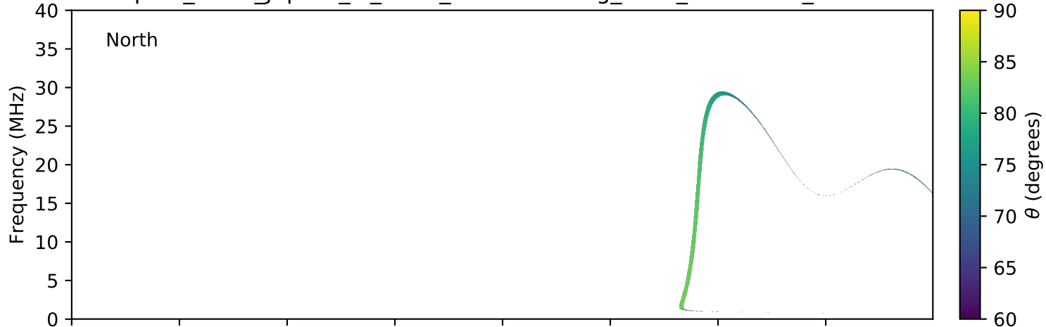
expres_earth_jupiter_io_isaac_lossc-wid1deg_3kev_20170511_v01.cdf
