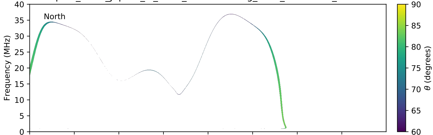
expres_earth_jupiter_io_isaac_lossc-wid1deg_3kev_20170510_v01.cdf
