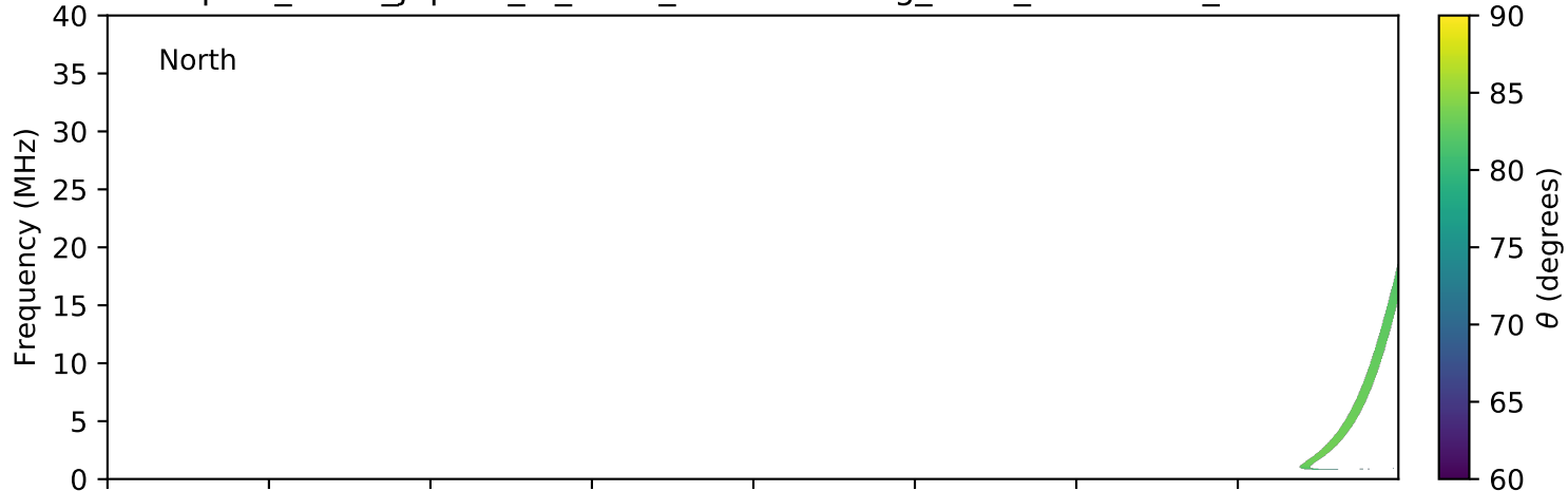
expres_earth_jupiter_io_isaac_lossc-wid1deg_3kev_20170509_v01.cdf
