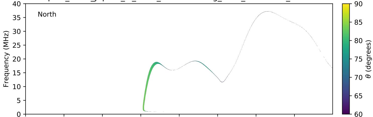
expres_earth_jupiter_io_isaac_lossc-wid1deg_3kev_20170506_v01.cdf
