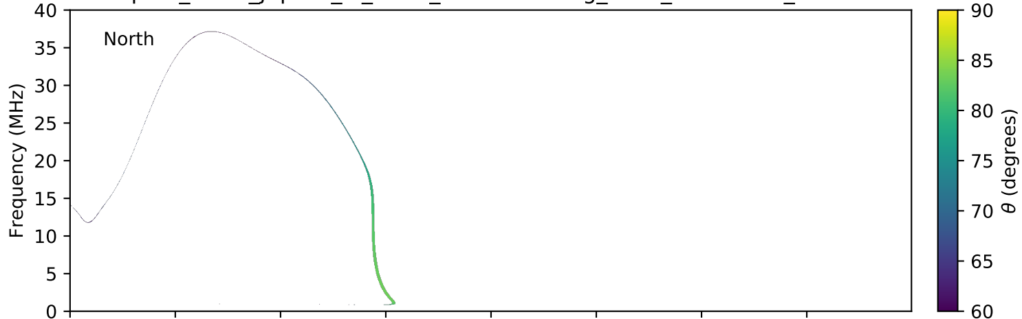
expres_earth_jupiter_io_isaac_lossc-wid1deg_3kev_20170505_v01.cdf
