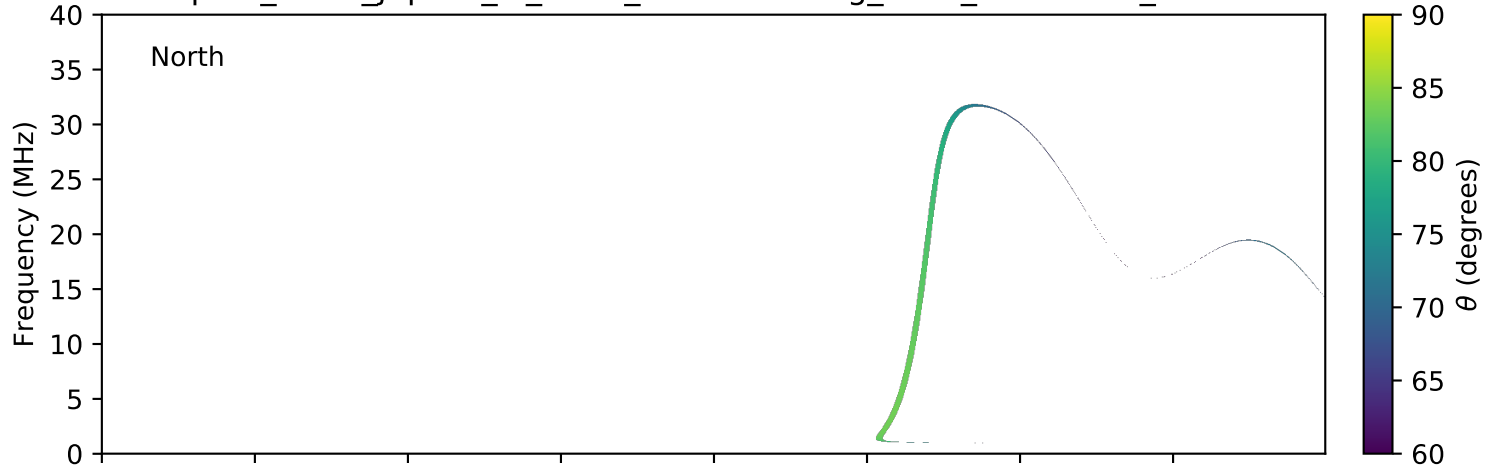
expres_earth_jupiter_io_isaac_lossc-wid1deg_3kev_20170504_v01.cdf
