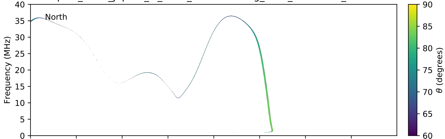
expres_earth_jupiter_io_isaac_lossc-wid1deg_3kev_20170503_v01.cdf
