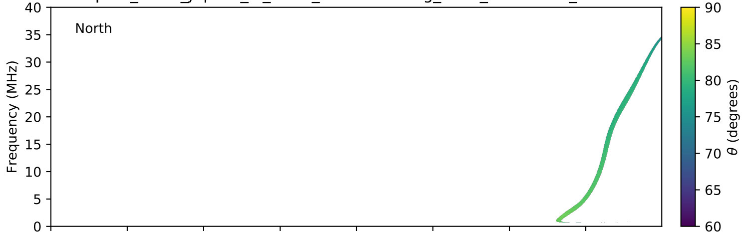
expres_earth_jupiter_io_isaac_lossc-wid1deg_3kev_20170502_v01.cdf
