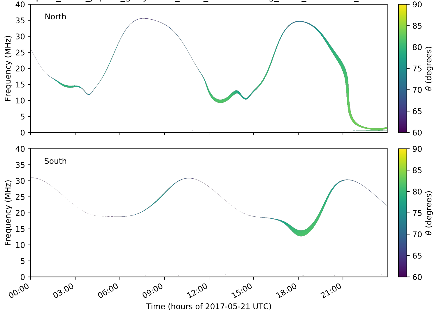
expres_earth_jupiter_ganymede_isaac_lossc-wid1deg_3kev_20170521_v01.cdf
