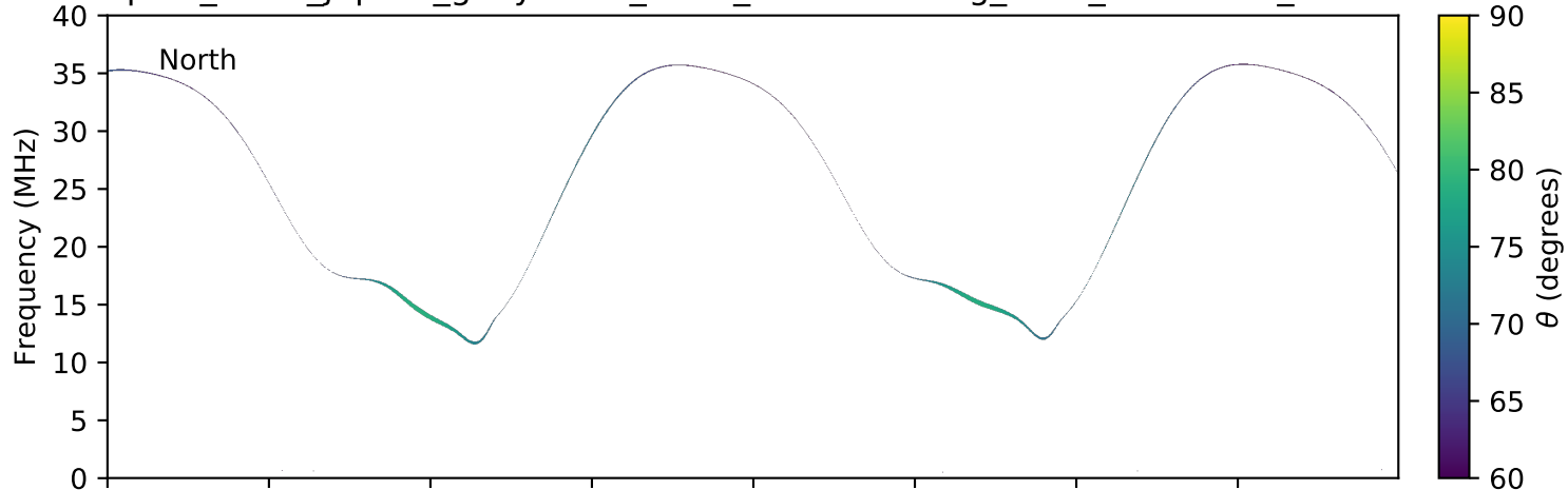
expres_earth_jupiter_ganymede_isaac_lossc-wid1deg_3kev_20170520_v01.cdf
