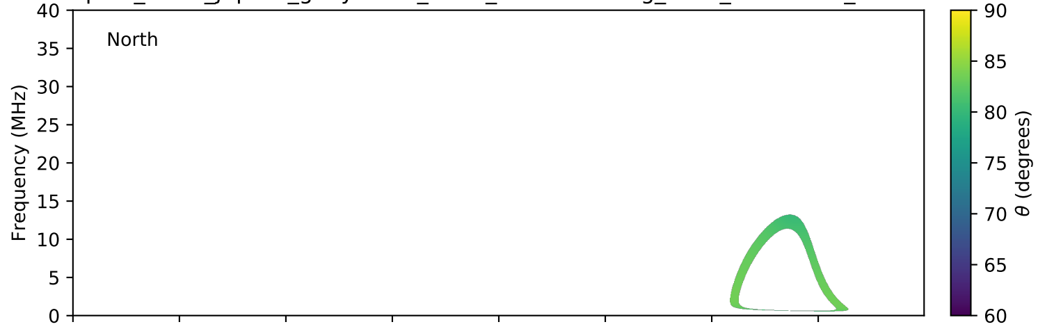
expres_earth_jupiter_ganymede_isaac_lossc-wid1deg_3kev_20170511_v01.cdf
