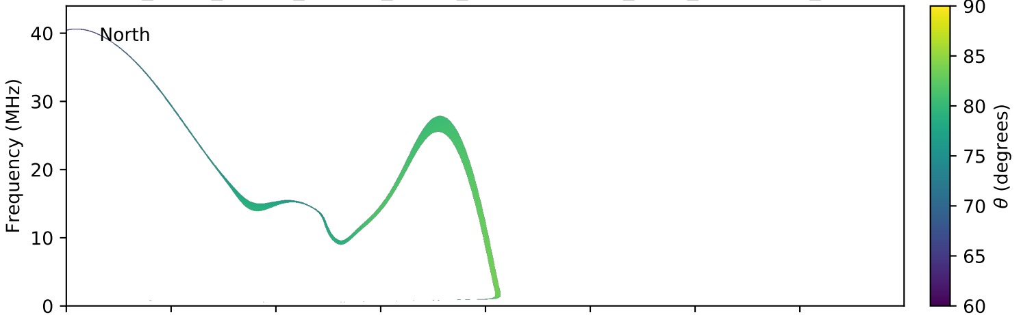
expres_earth_jupiter_europa_jrm09_lossc-wid1deg_3kev_20170530_v01.cdf
