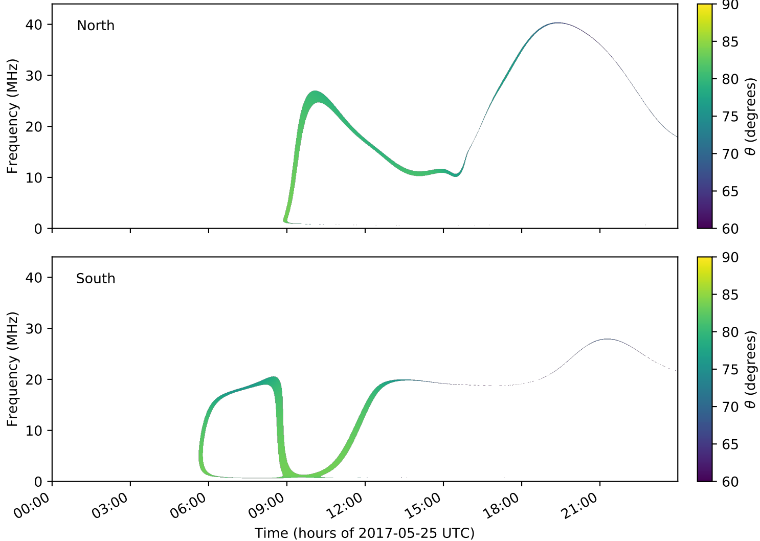
expres_earth_jupiter_europa_jrm09_lossc-wid1deg_3kev_20170525_v01.cdf
