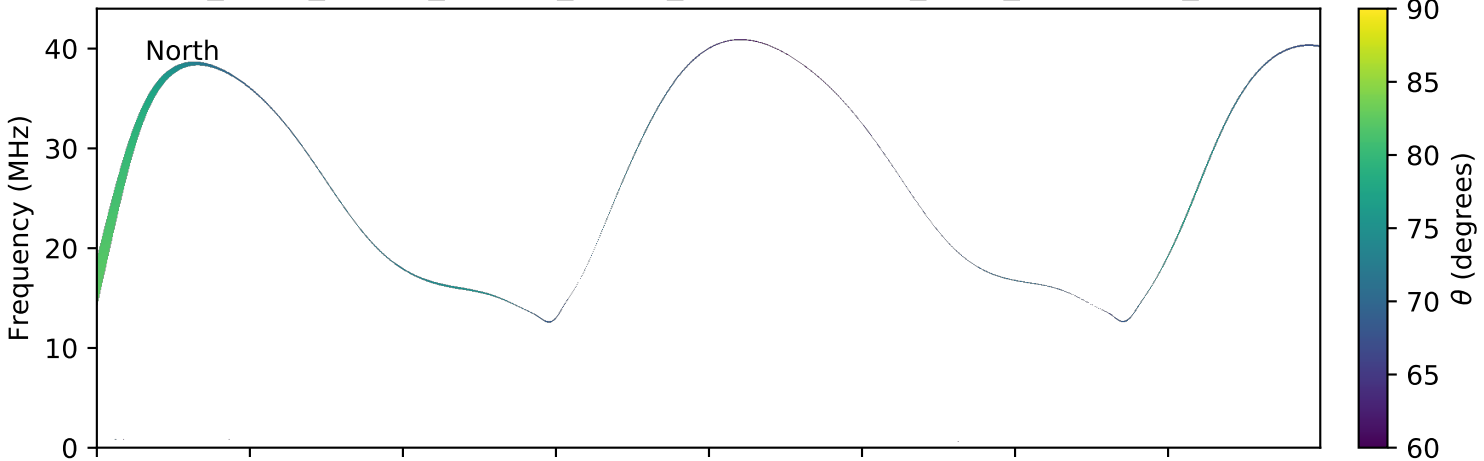
expres_earth_jupiter_europa_jrm09_lossc-wid1deg_3kev_20170522_v01.cdf
