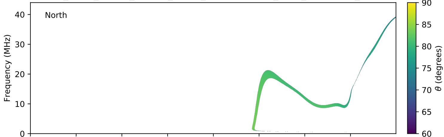
expres_earth_jupiter_europa_jrm09_lossc-wid1deg_3kev_20170507_v01.cdf
