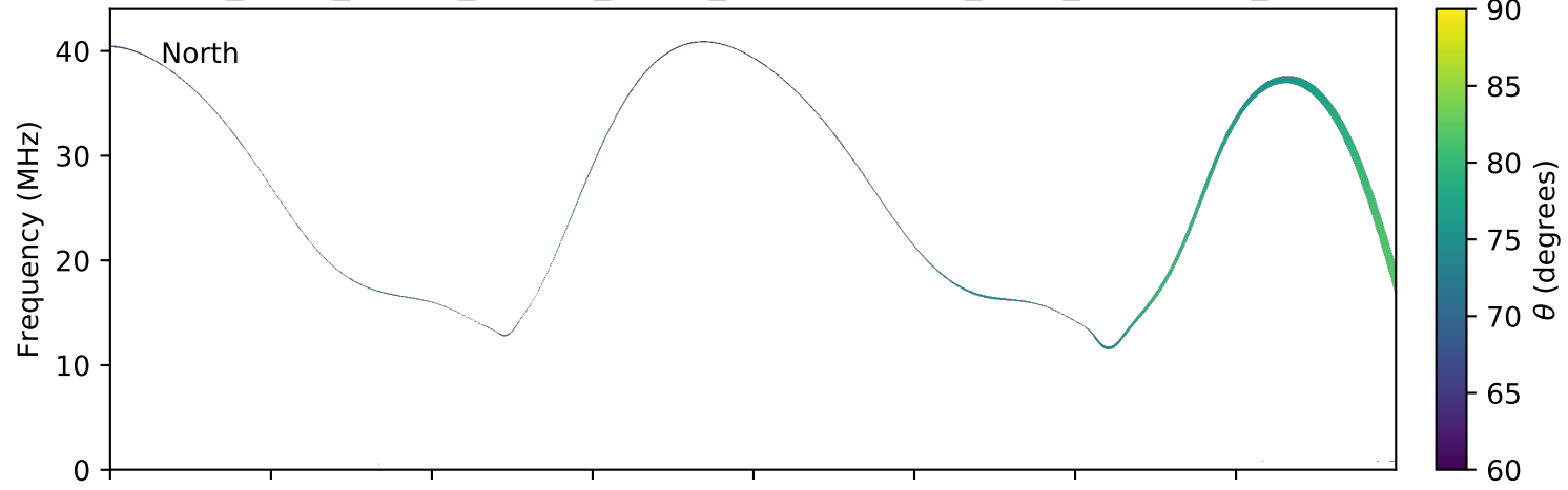
expres_earth_jupiter_europa_jrm09_lossc-wid1deg_3kev_20170501_v01.cdf
