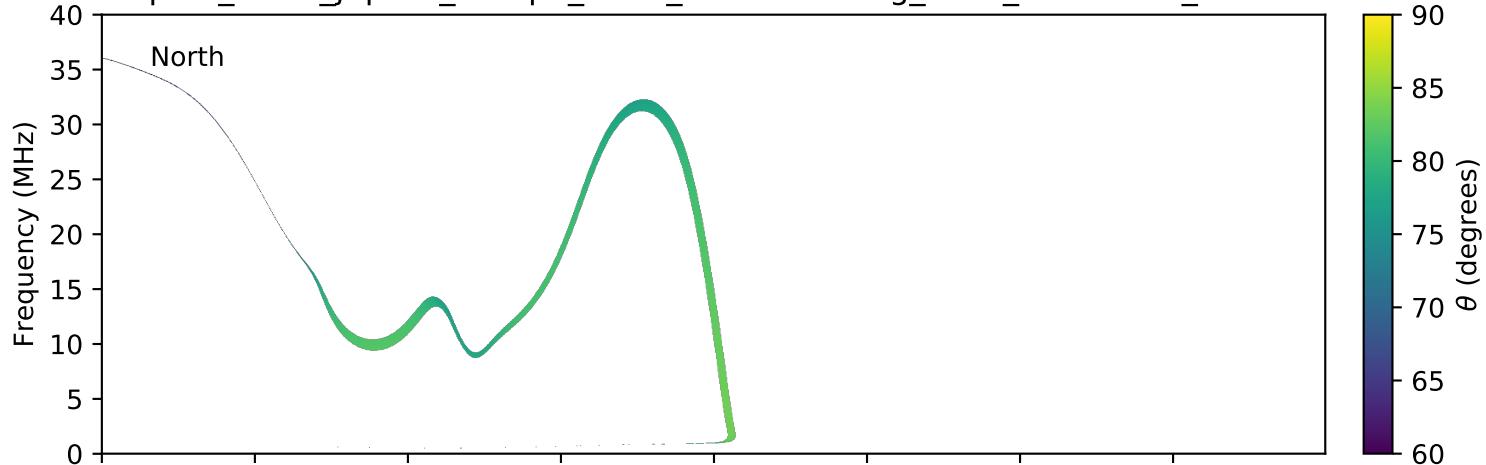
expres_earth_jupiter_europa_isaac_lossc-wid1deg_3kev_20170530_v01.cdf
