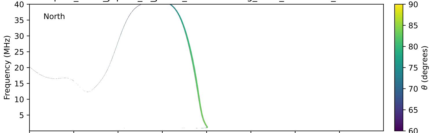
expres_earth_jupiter_io_jrm33_lossc-wid1deg_3kev_20170327_v11.cdf
