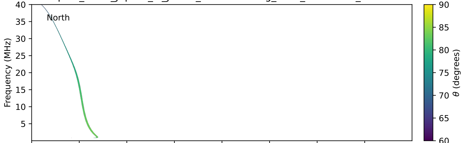
expres_earth_jupiter_io_jrm33_lossc-wid1deg_3kev_20170322_v11.cdf
