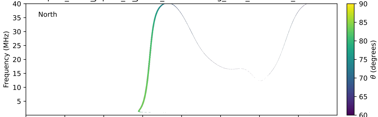
expres_earth_jupiter_io_jrm33_lossc-wid1deg_3kev_20170314_v11.cdf
