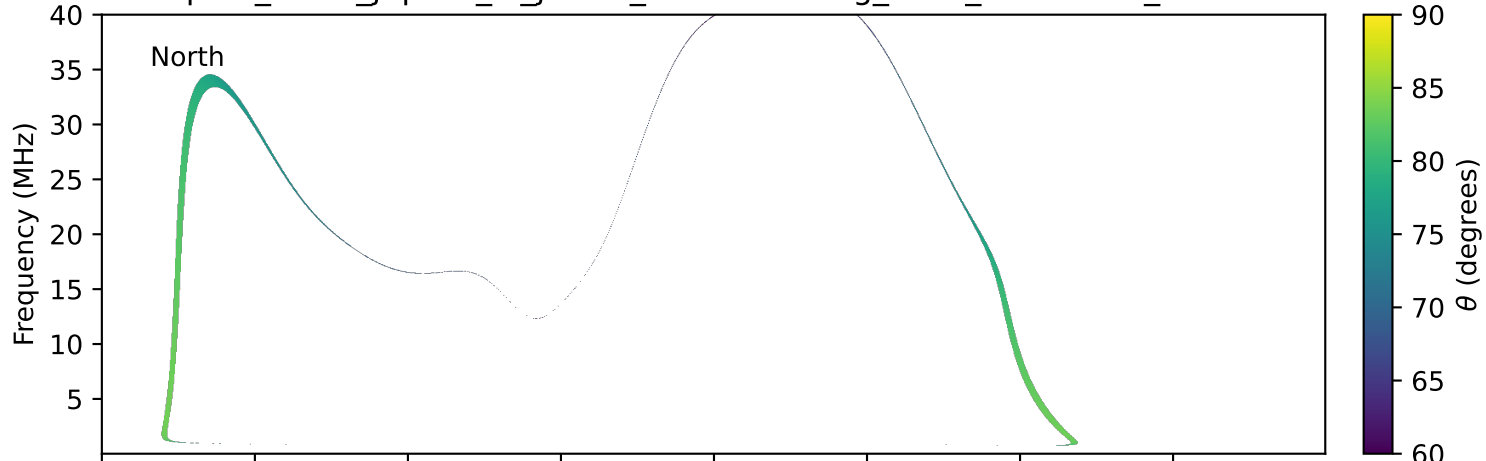
expres_earth_jupiter_io_jrm33_lossc-wid1deg_3kev_20170309_v11.cdf
