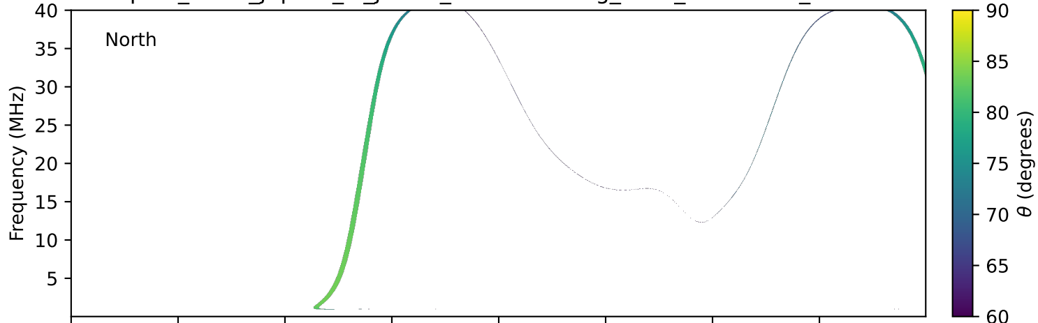
expres_earth_jupiter_io_jrm33_lossc-wid1deg_3kev_20170307_v11.cdf
