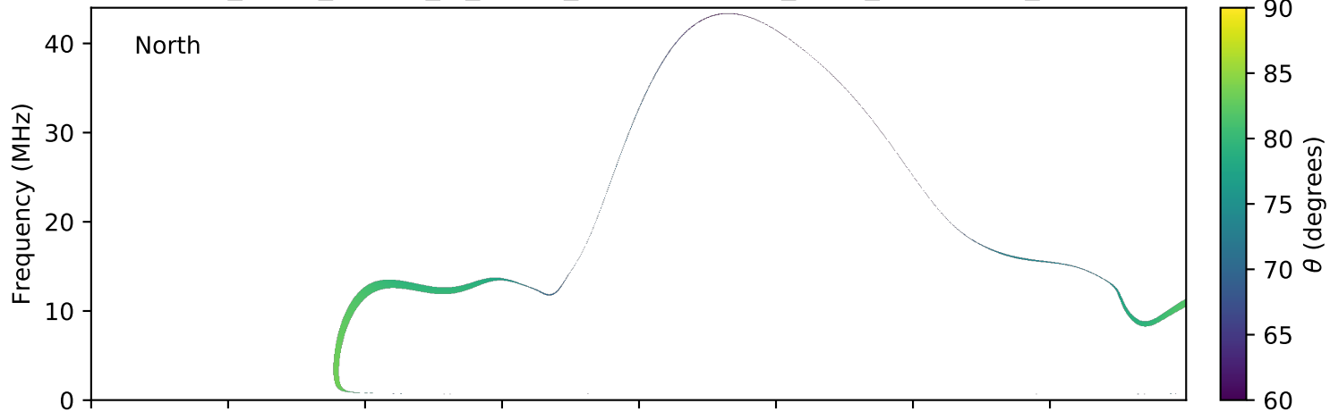
expres_earth_jupiter_io_jrm09_lossc-wid1deg_3kev_20170330_v01.cdf
