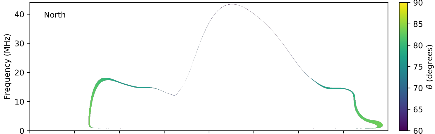
expres_earth_jupiter_io_jrm09_lossc-wid1deg_3kev_20170323_v01.cdf
