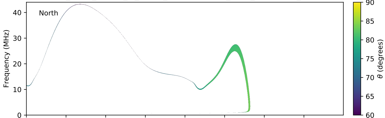
expres_earth_jupiter_io_jrm09_lossc-wid1deg_3kev_20170318_v01.cdf
