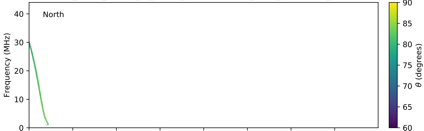
expres_earth_jupiter_io_jrm09_lossc-wid1deg_3kev_20170308_v01.cdf
