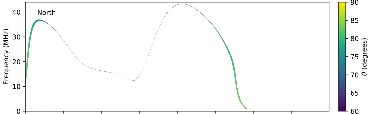
expres_earth_jupiter_io_jrm09_lossc-wid1deg_3kev_20170302_v01.cdf
