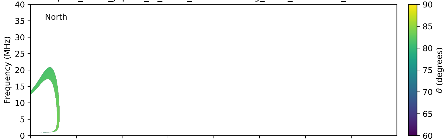
expres_earth_jupiter_io_isaac_lossc-wid1deg_3kev_20170331_v01.cdf
