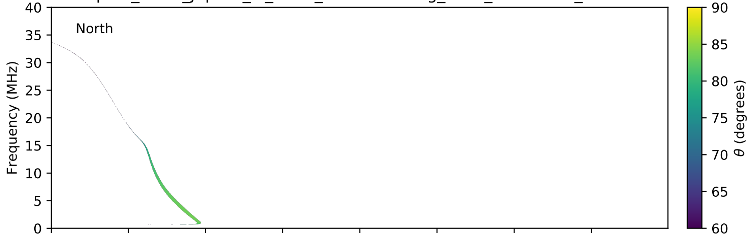
expres_earth_jupiter_io_isaac_lossc-wid1deg_3kev_20170329_v01.cdf
