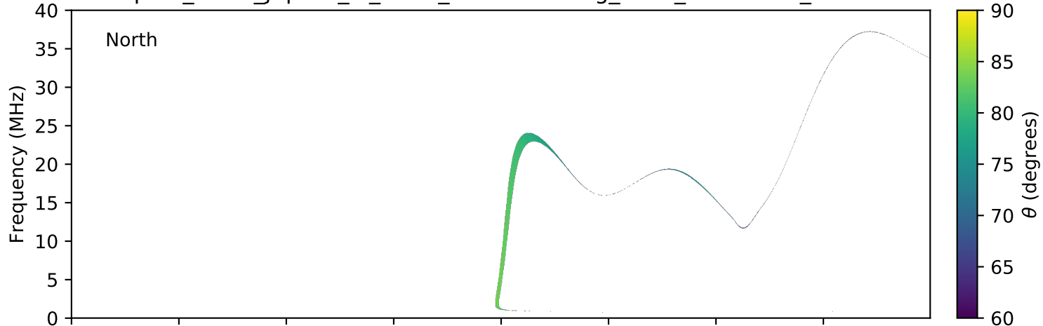
expres_earth_jupiter_io_isaac_lossc-wid1deg_3kev_20170328_v01.cdf
