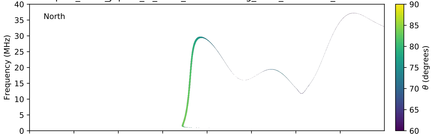
expres_earth_jupiter_io_isaac_lossc-wid1deg_3kev_20170321_v01.cdf
