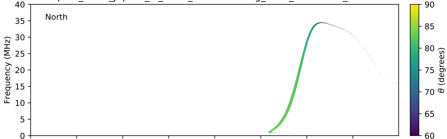
expres_earth_jupiter_io_isaac_lossc-wid1deg_3kev_20170319_v01.cdf
