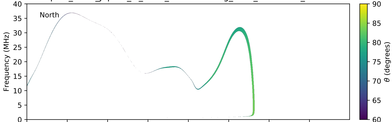
expres_earth_jupiter_io_isaac_lossc-wid1deg_3kev_20170318_v01.cdf
