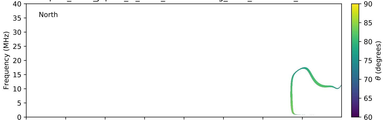
expres_earth_jupiter_io_isaac_lossc-wid1deg_3kev_20170317_v01.cdf
