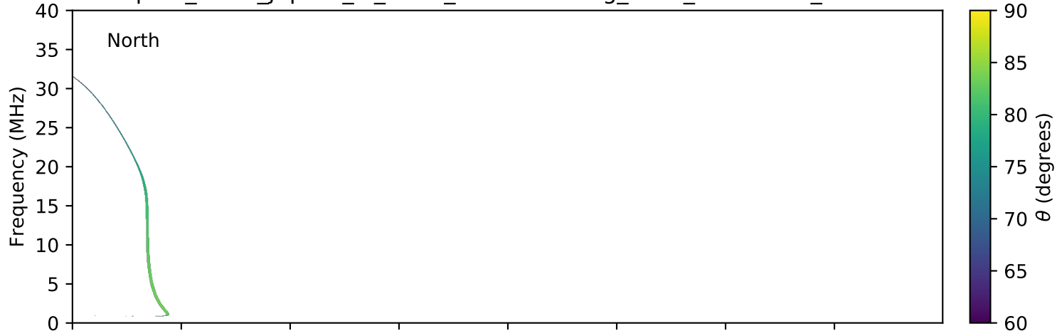
expres_earth_jupiter_io_isaac_lossc-wid1deg_3kev_20170315_v01.cdf
