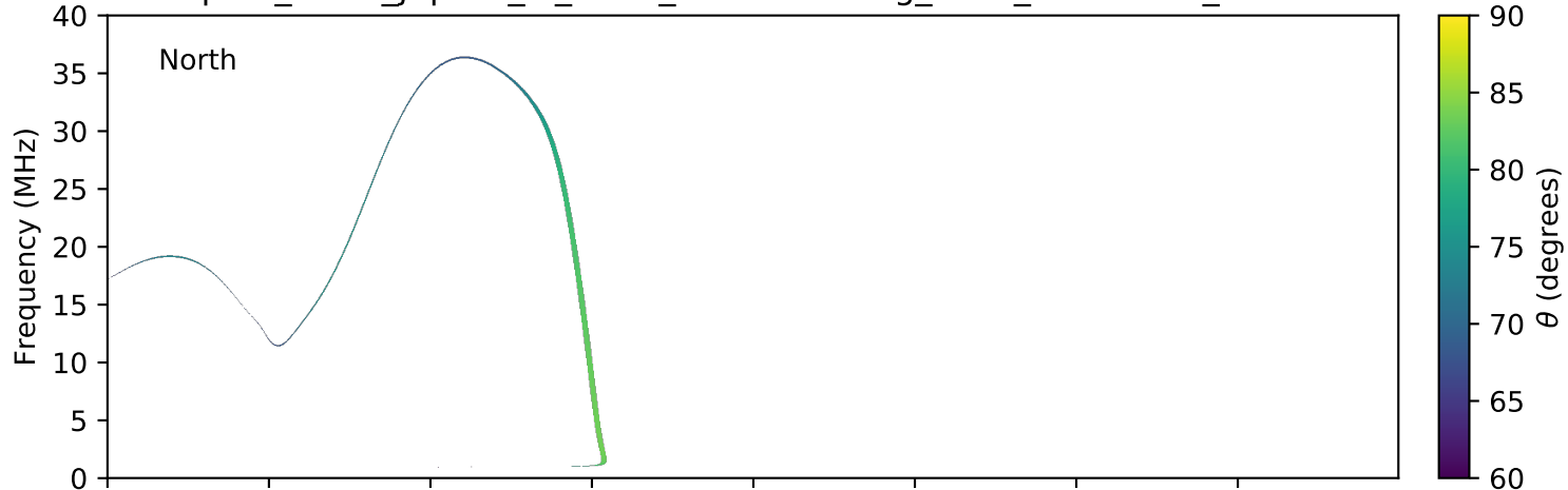
expres_earth_jupiter_io_isaac_lossc-wid1deg_3kev_20170313_v01.cdf
