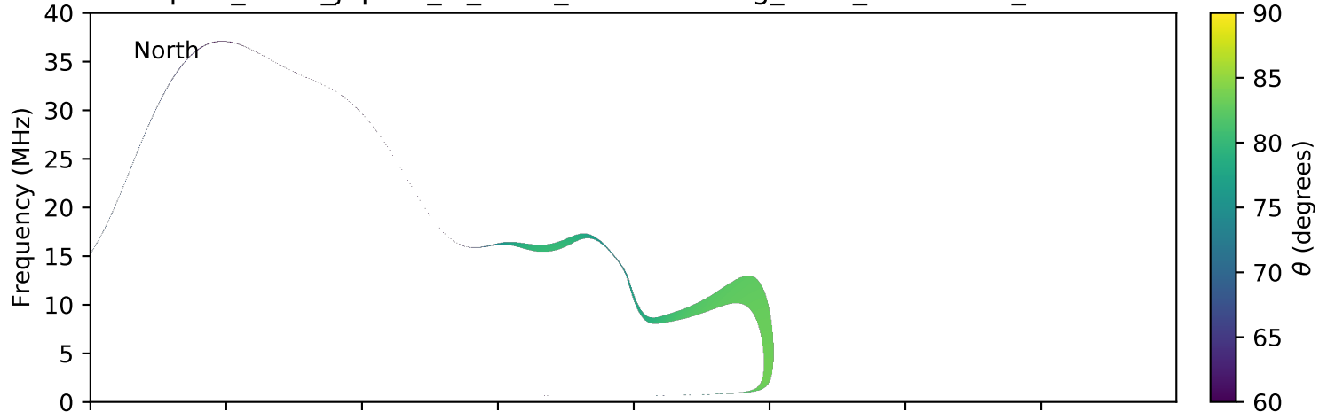
expres_earth_jupiter_io_isaac_lossc-wid1deg_3kev_20170311_v01.cdf
