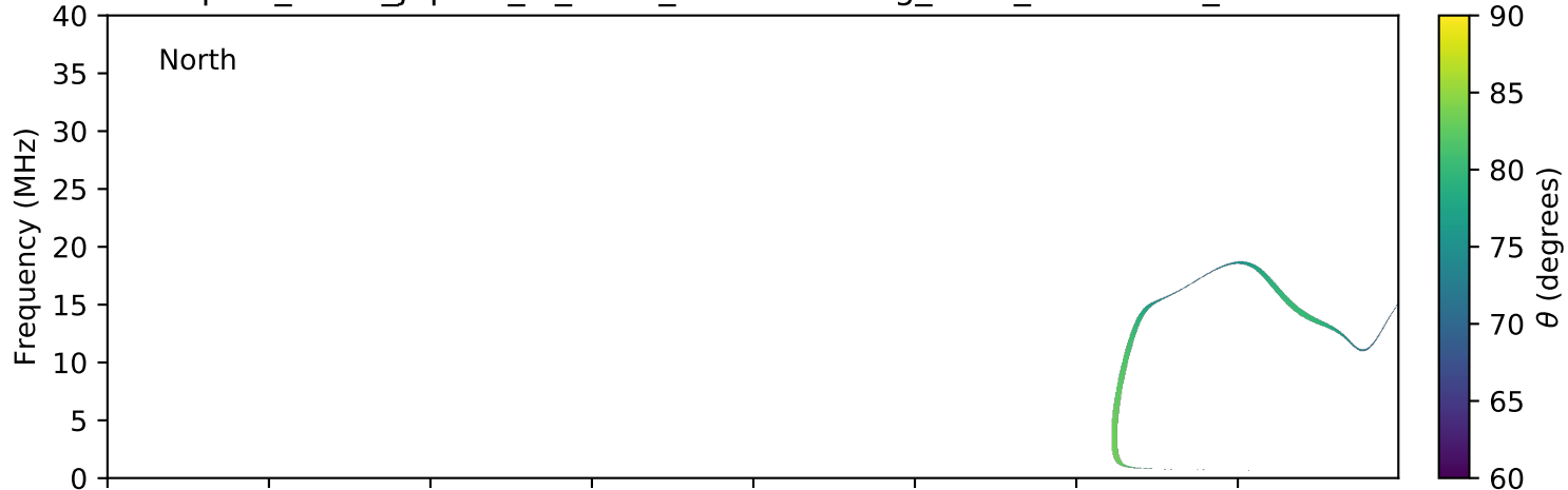
expres_earth_jupiter_io_isaac_lossc-wid1deg_3kev_20170310_v01.cdf
