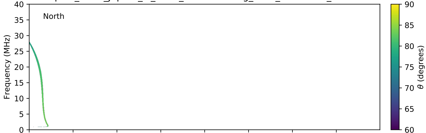
expres_earth_jupiter_io_isaac_lossc-wid1deg_3kev_20170308_v01.cdf
