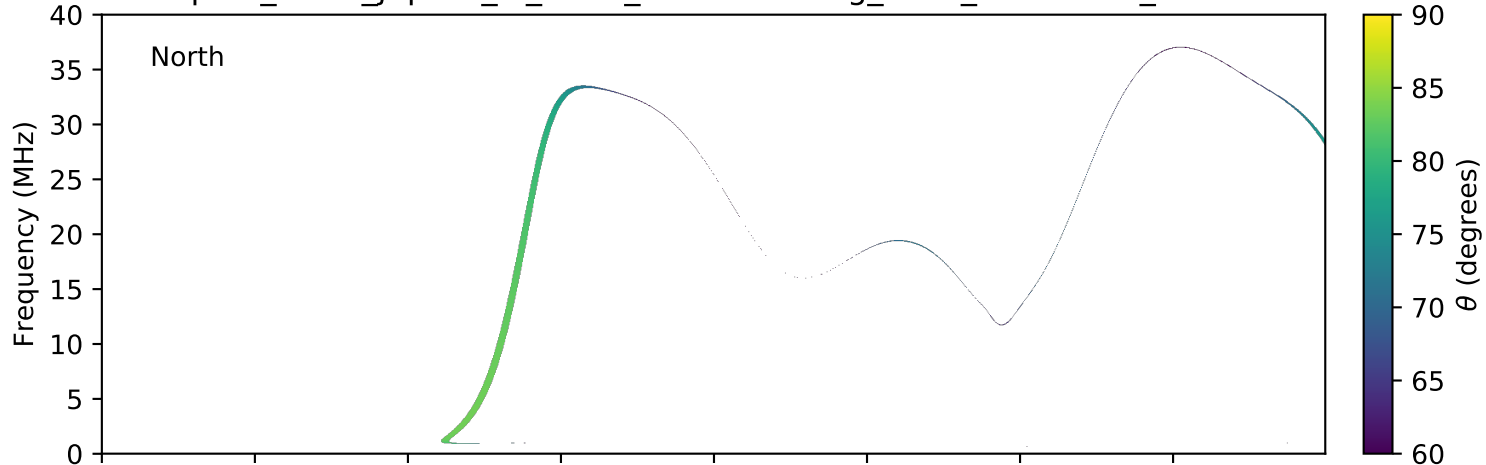
expres_earth_jupiter_io_isaac_lossc-wid1deg_3kev_20170307_v01.cdf
