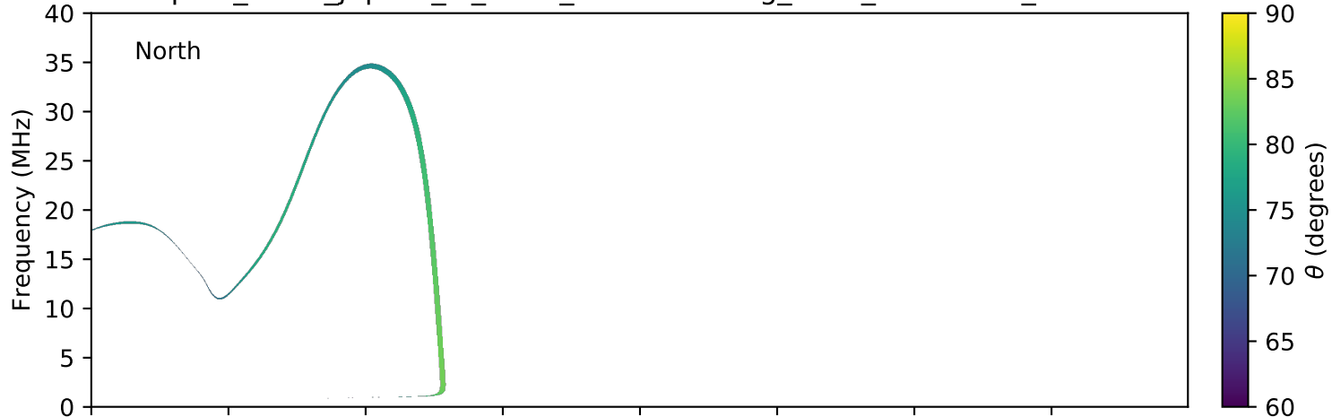
expres_earth_jupiter_io_isaac_lossc-wid1deg_3kev_20170306_v01.cdf
