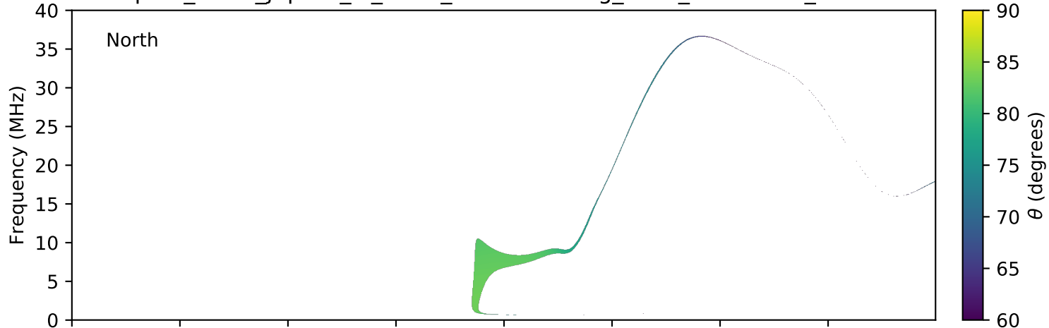
expres_earth_jupiter_io_isaac_lossc-wid1deg_3kev_20170305_v01.cdf
