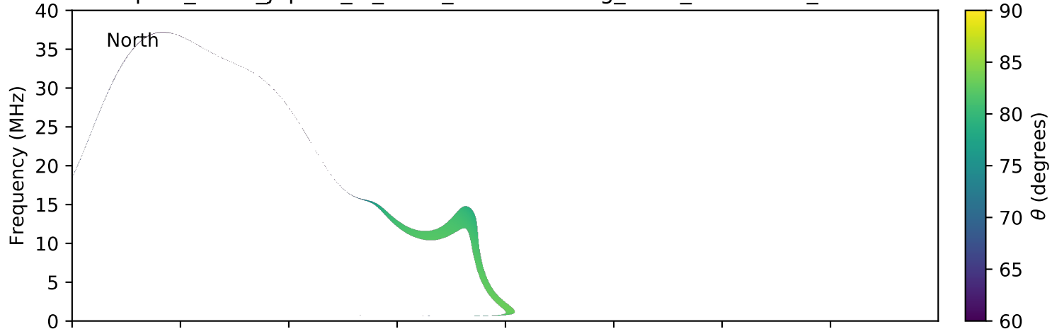
expres_earth_jupiter_io_isaac_lossc-wid1deg_3kev_20170304_v01.cdf
