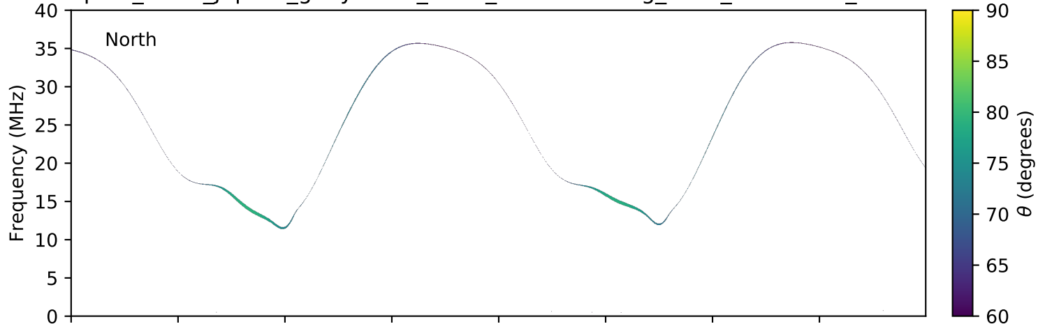
expres_earth_jupiter_ganymede_isaac_lossc-wid1deg_3kev_20170331_v01.cdf
