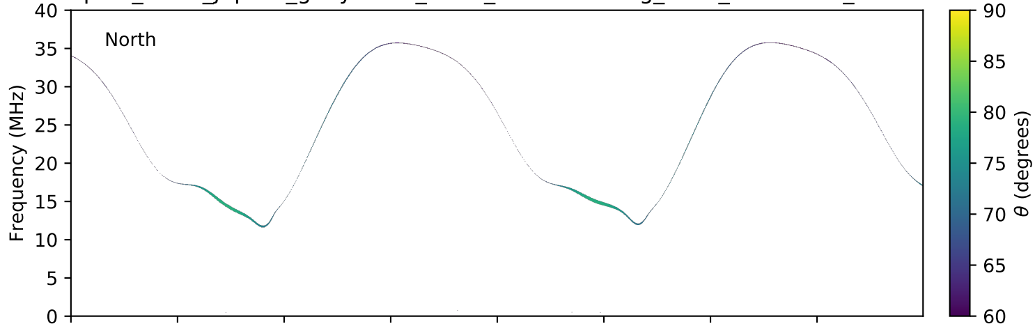
expres_earth_jupiter_ganymede_isaac_lossc-wid1deg_3kev_20170324_v01.cdf
