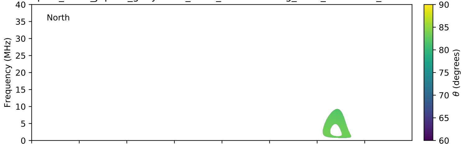
expres_earth_jupiter_ganymede_isaac_lossc-wid1deg_3kev_20170322_v01.cdf
